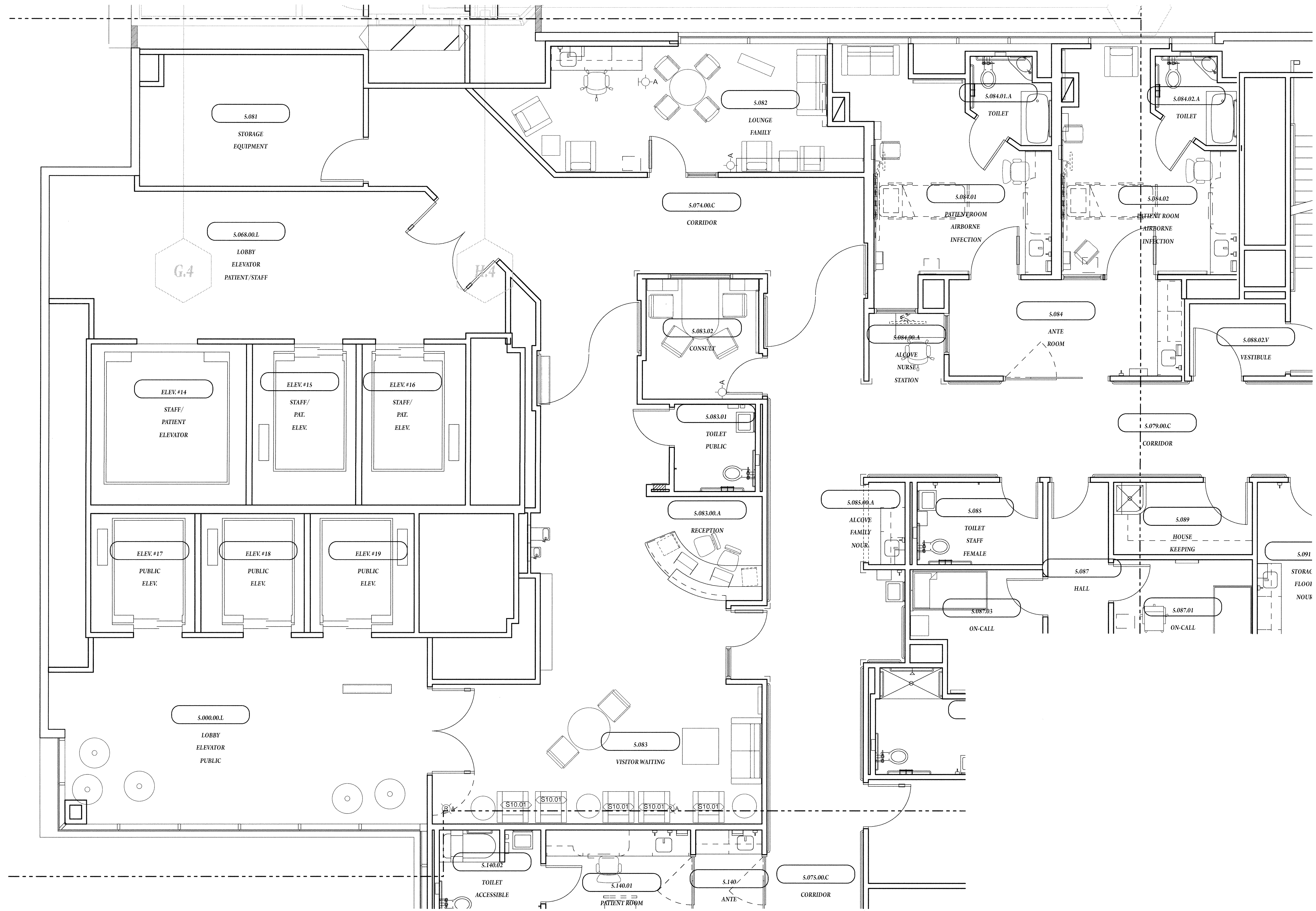
B6 Furniture Plan SCALE: 1/4" = 1'-0"
