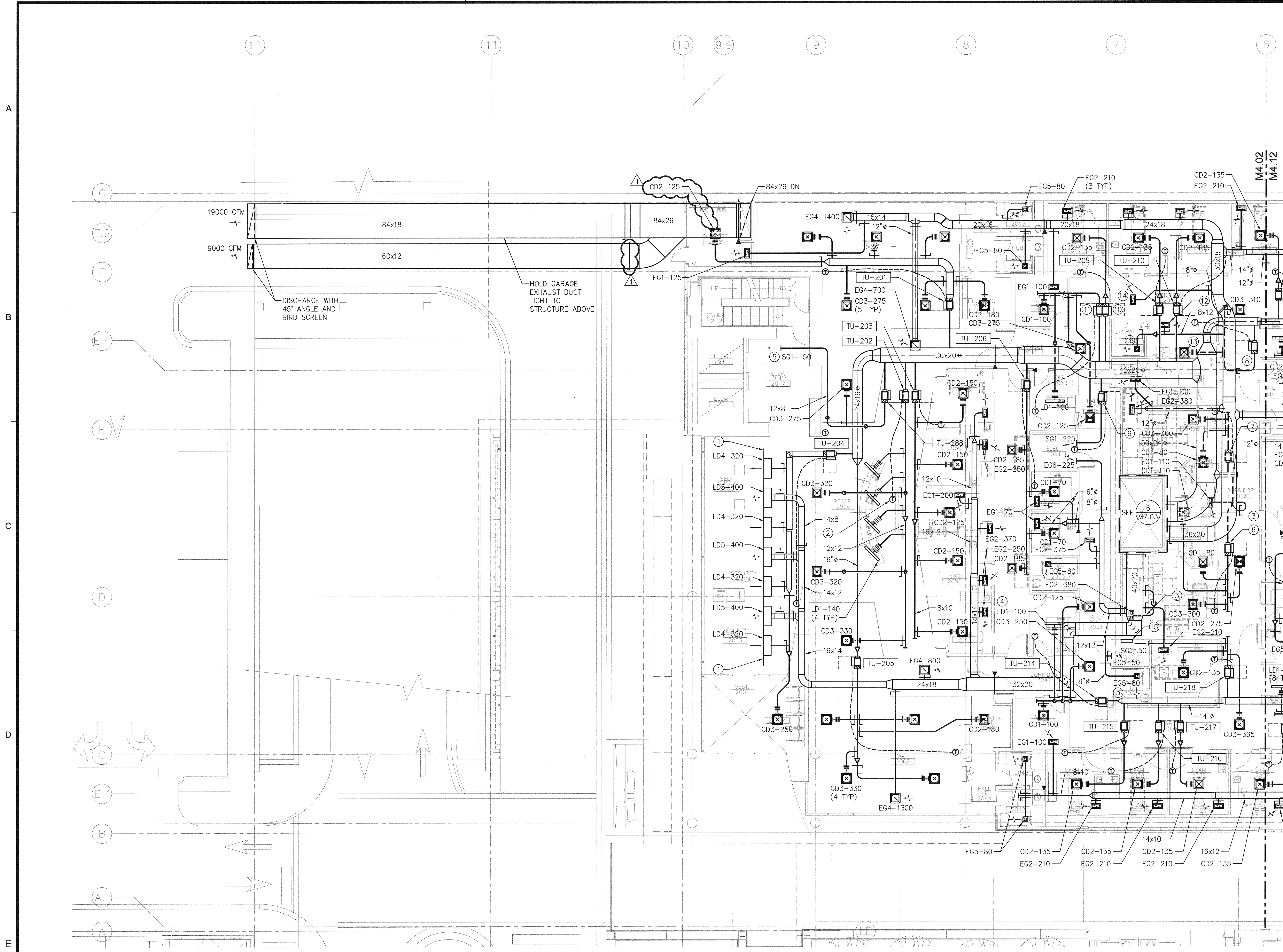
2ND FLOOR PLAN - SOUTH - HVAC SCALE: 1/8"=1'-0"
