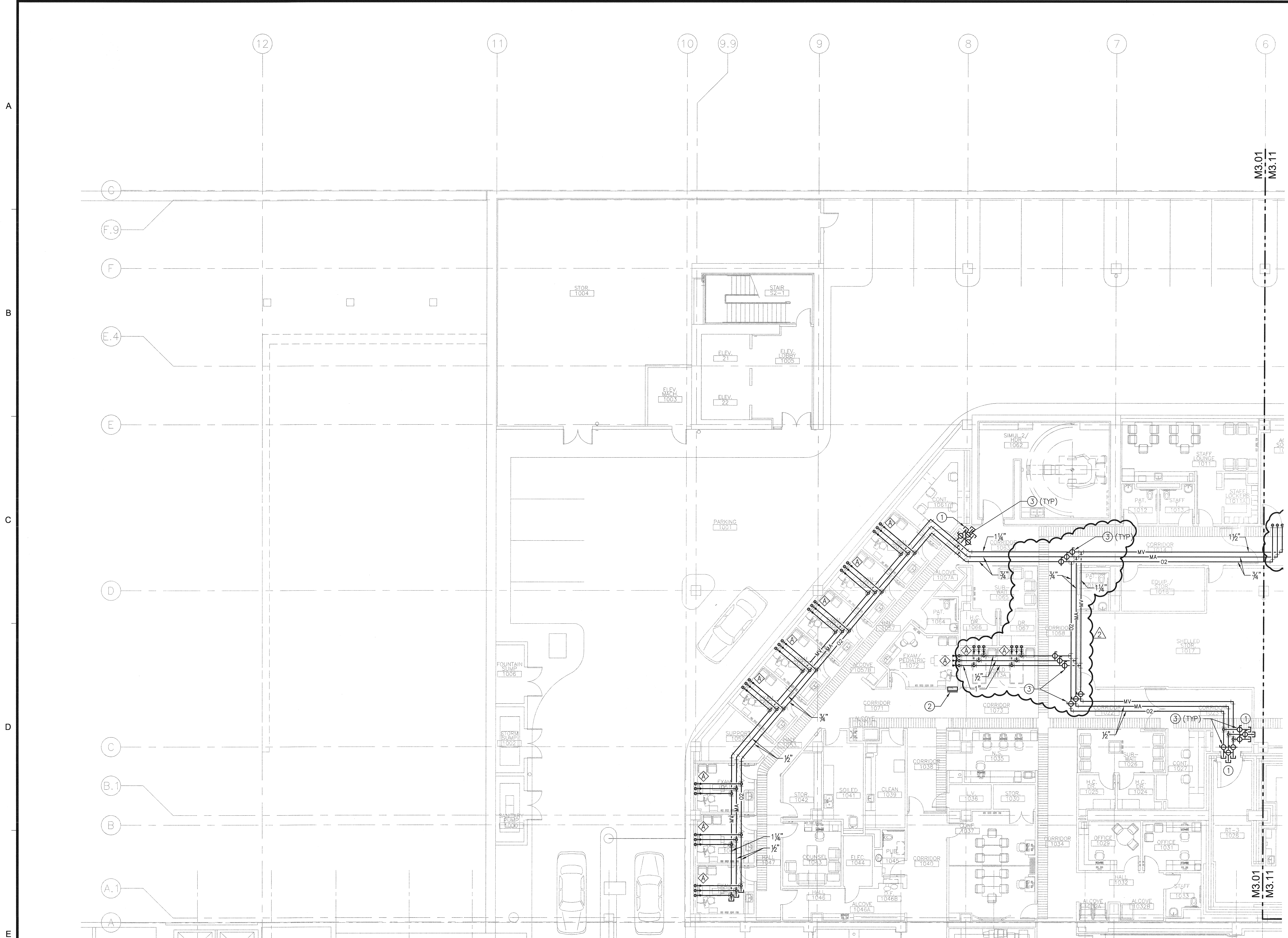
1ST FLOOR PLAN - SOUTH - MEDICAL GAS PIPING SCALE: 1/8"=1'-0"
