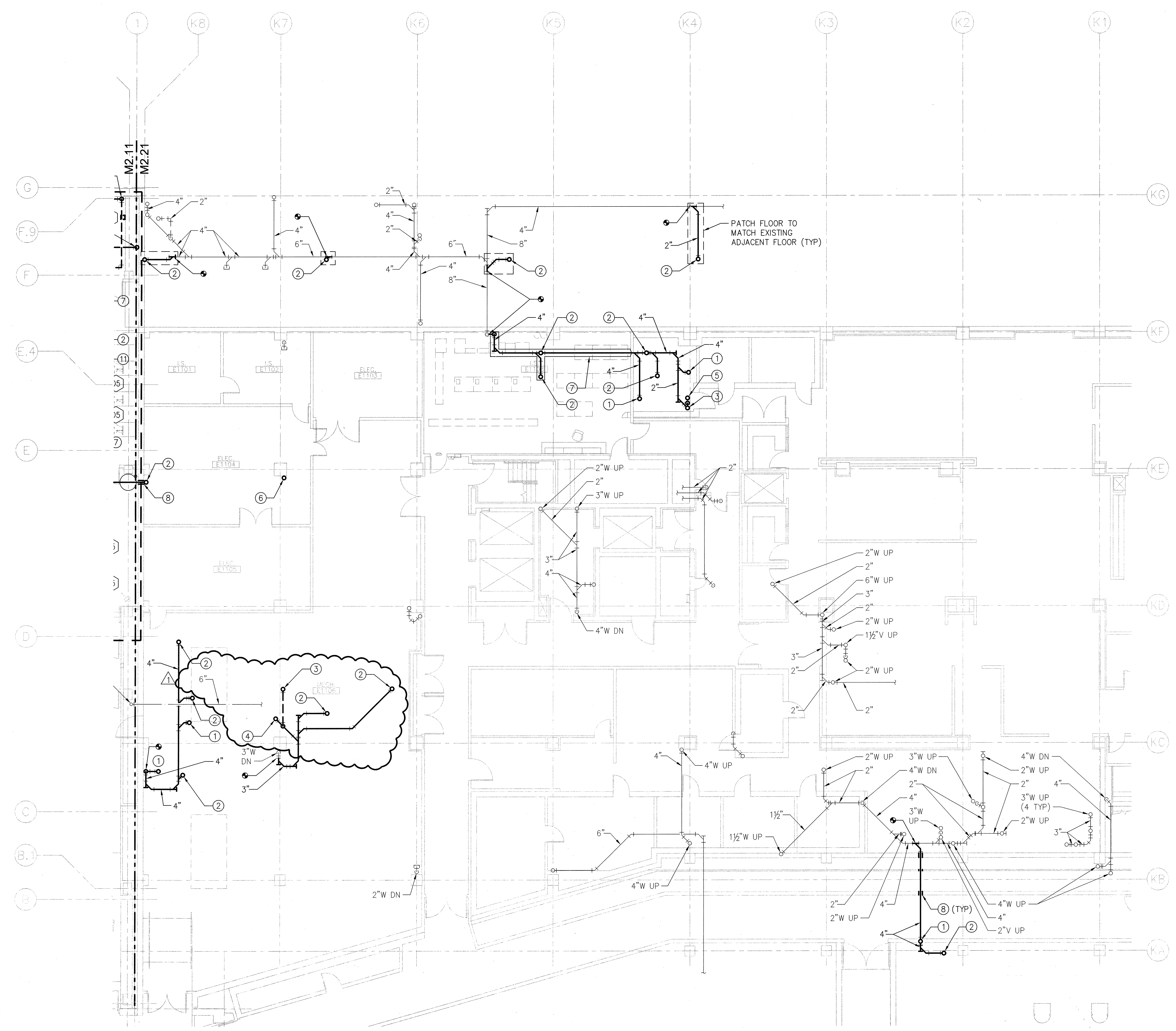
1ST FLOOR PLAN - K WING REMODEL - PLUMBING SCALE: 1/8"=1'-0"
