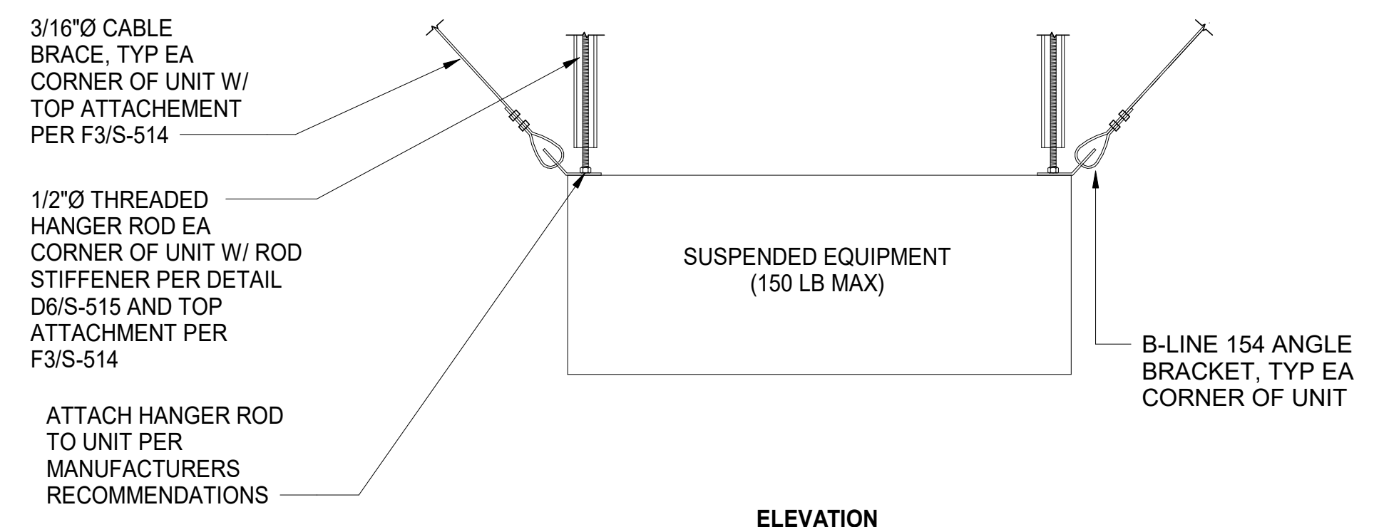
B4 TYPICAL SUSPENDED EQUIPMENT BRACING DETAIL S-514 SCALE: 1" = 1'-0"
