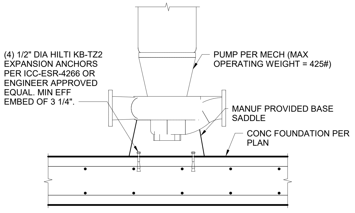
E6 TYP VERTICAL PUMP ANCHORAGE S-514 SCALE: 1" = 1'-0"
