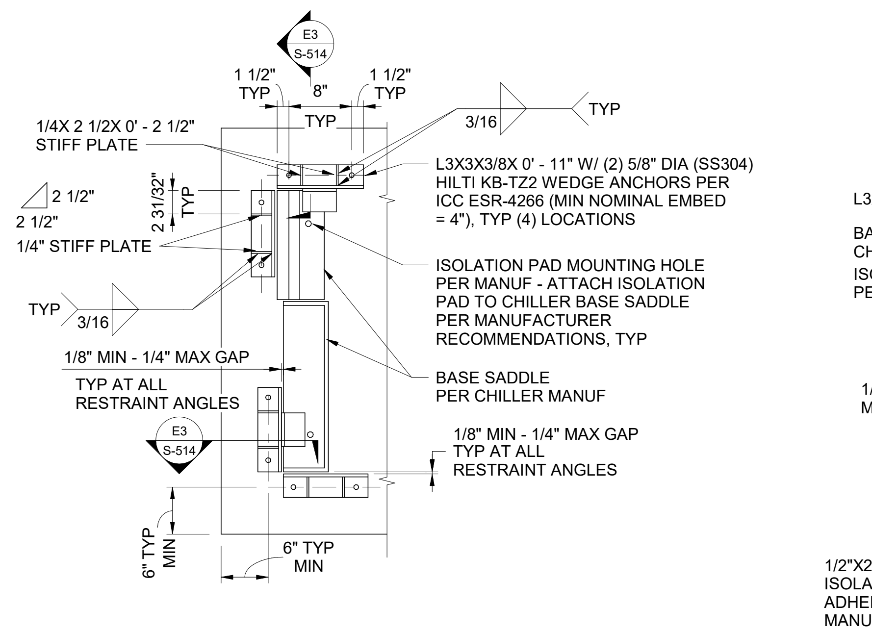
E1 CHILLER UNIT ANCHORAGE DETAIL S-514 SCALE: 1" = 1'-0"
