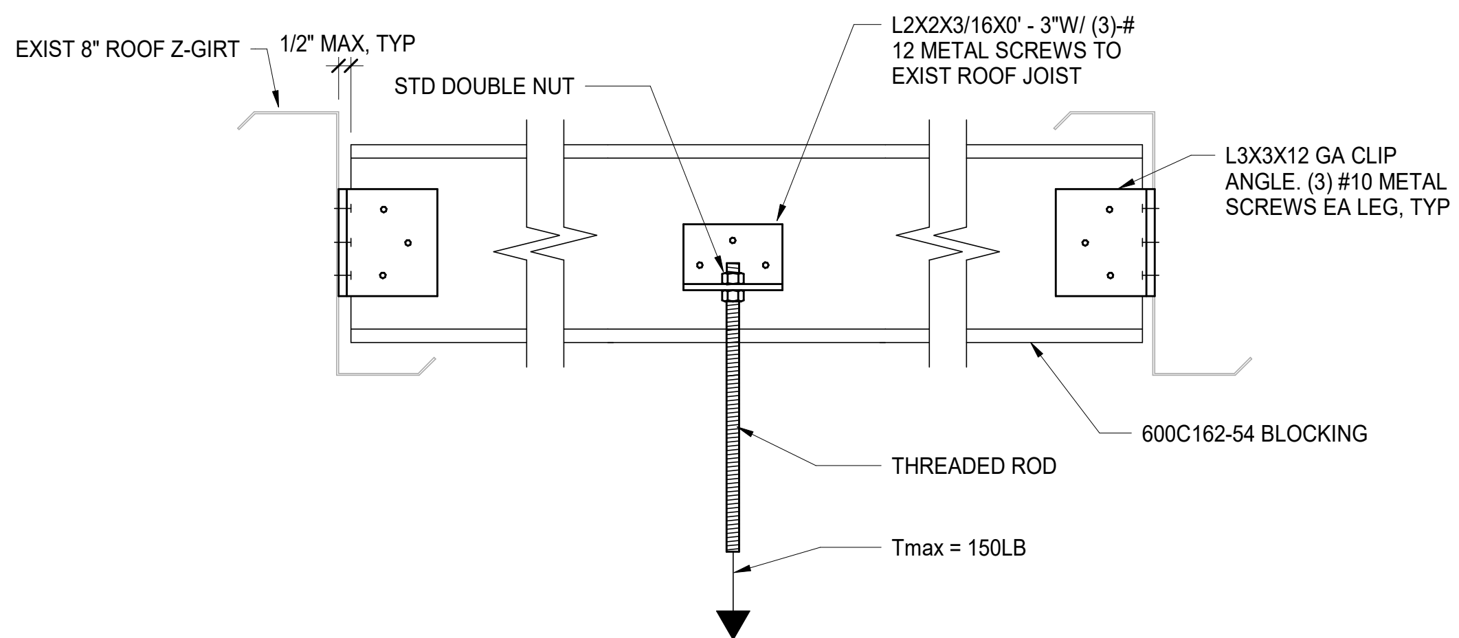
F3 TYPICAL ROOF JOIST HANGER ATTACHMENT ROD DETAIL S-514 SCALE: 3" = 1'-0"
