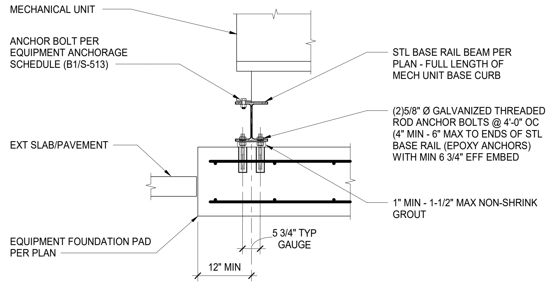
B1 MECH UNIT STEEL BASE FRAME S-514 SCALE: 1" = 1'-0"
