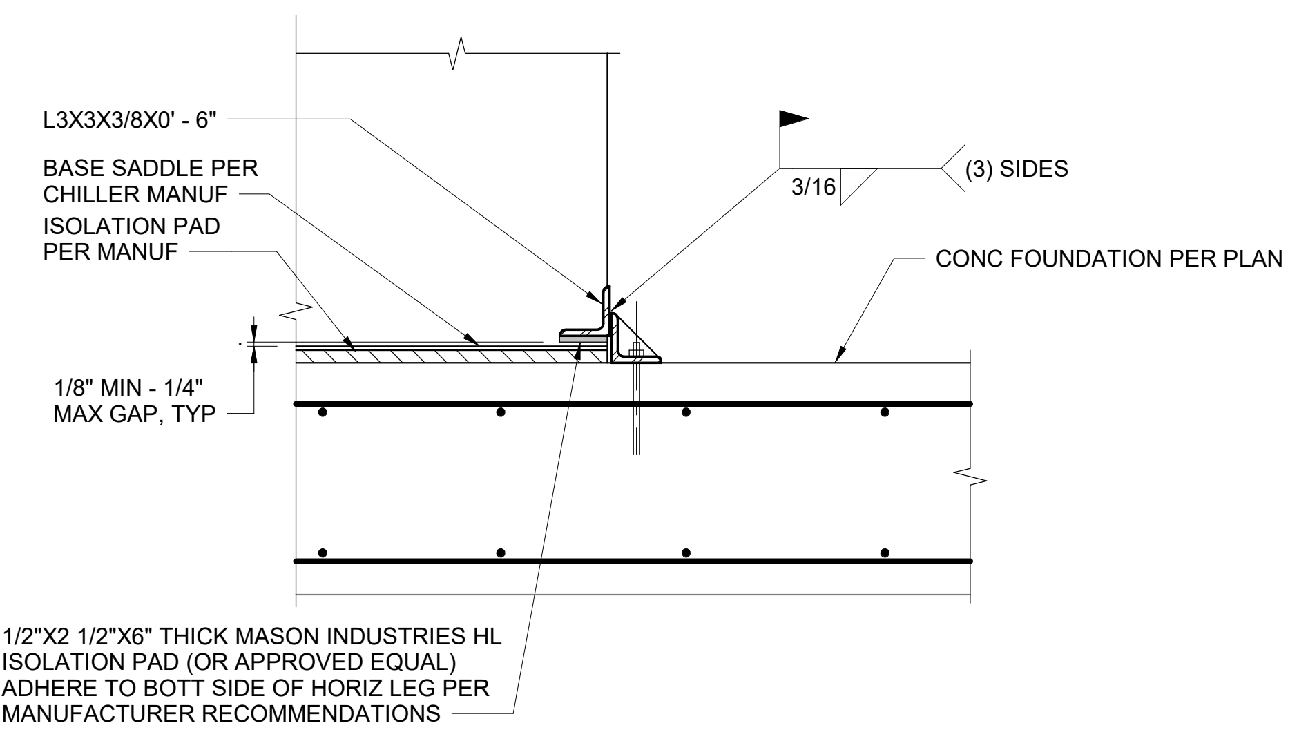
E3 ANCHORAGE SECTION S-514 SCALE: 1 1/2" = 1'-0"
